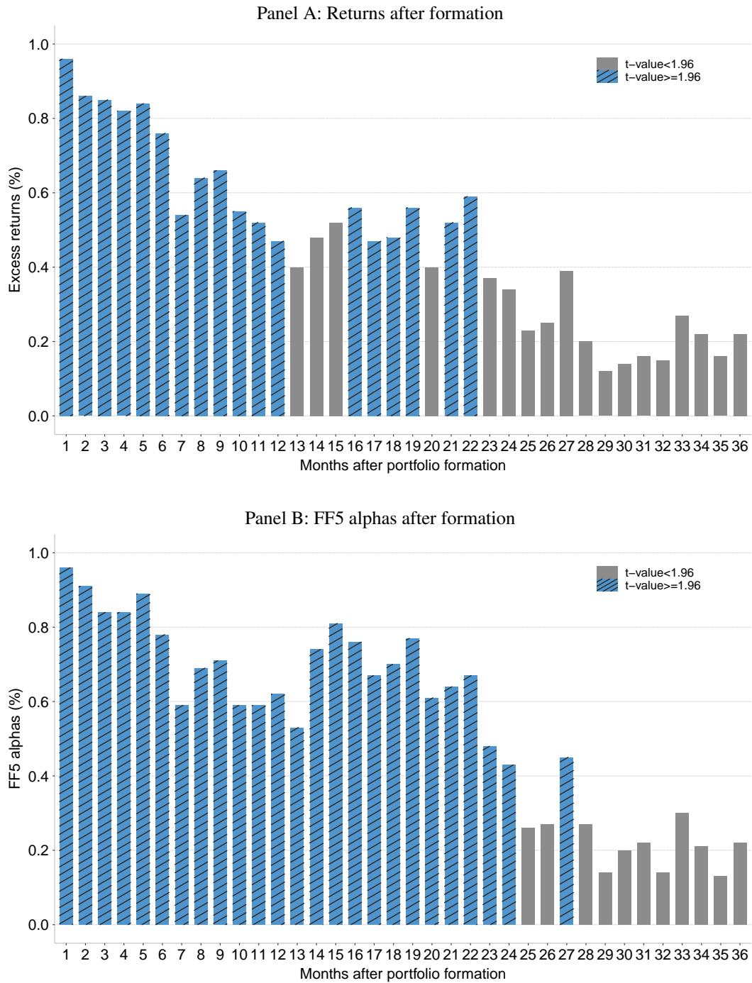
Figure 3: PEAR beta spread portfolio performance after formation
